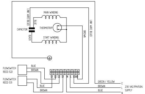
Twin Pumps Fig. 14
