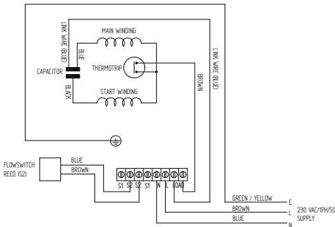
Single Pumps Fig. 13
