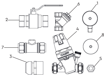
Package 1b Upstream line-in kit 35mm, 42mm, 54mm variants Fig. 1b
