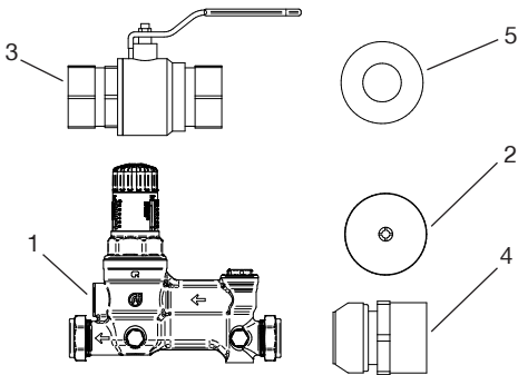
Package 1a Monobloc 22/28mm Upstream line-in kit Fig. 1a Or
