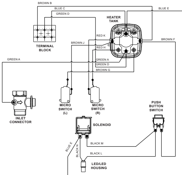
Internal Wiring Diagram
