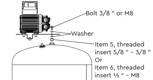
Pump mounting for 200, 250, 300 & 450 litre vessels. Fig. 13
