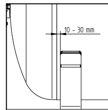
Mounting cradle placement Fig. 18b
