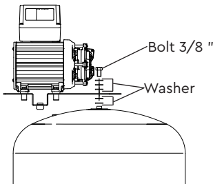
Pump mounting for 100, 130 litre vessels Fig. 12
