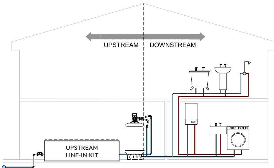
Fig. 6 System designation
