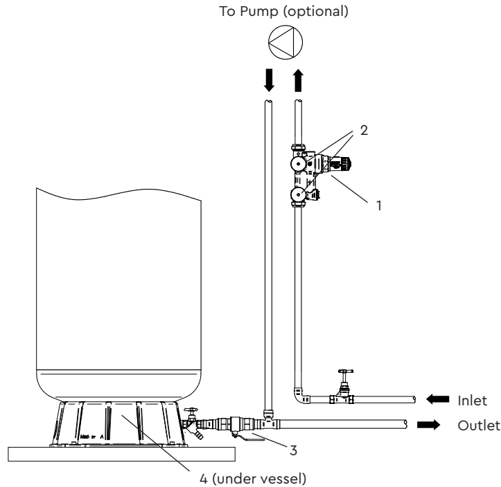
Fig. 3 Monobloc 22/28mm Installation
