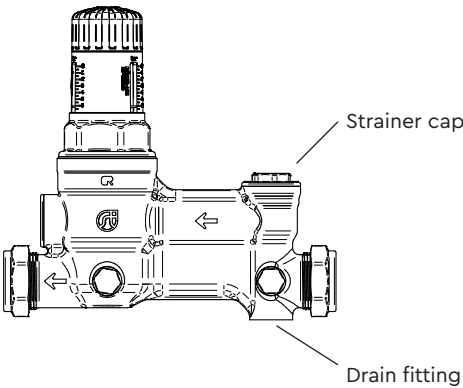
Fig. 4 Strainer cap and drain fittings
